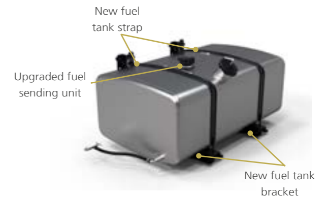
New fuel tank design is applicable to 8L models.
